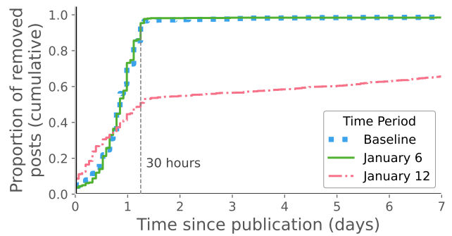
Figure 1: Post lifetime: Days between posting and last observation. In the baseline and January 6 periods, nearly all last observations were at most 30 h after posting, whereas during the January 12 period, much older posts were removed. The sharp pivot at 30 h suggests different removal processes.
